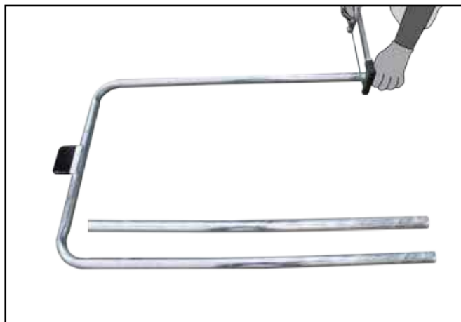
I. Using a hacksaw or similar, carefully cut through the top, bottom tubes and mid rail as shown. For galvanised assemblies, spray with Galvafruid or similar to prevent corrosion.
