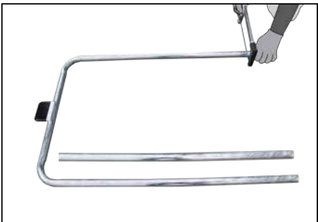
I. Using a hacksaw or similar carefully cut through the top and bottom tubes and mid rail as shown. For galvanised assemblies, spray with Galvafoid or similar to prevent corrosion.
