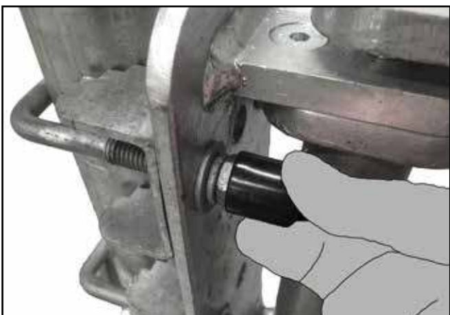
O. Ensure all nuts and grub screws (excluding adjustment screw) on the gate are torqued to 39Nm. Finally, place black caps over nuts. Ensure that the structure to which the gate is attached to is sturdy, does not rotate and nuts and grub screws are torqued as per manufacturers guidelines.
