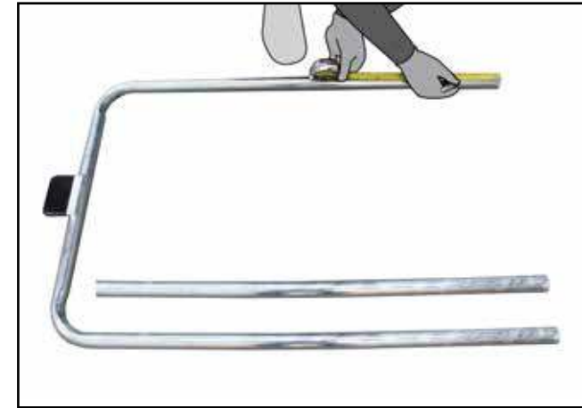
H. Measure the distance recorded in point (f) and mark the gate top and bottom tubes and mid rail as shown.
