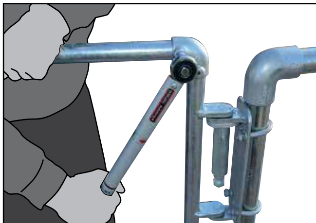
J. Carefully re-position the gate top and bottom tubes into the cast fittings. Ensure the striking plate is on the correct side of the Support Leg/Structure. Use a spirit level to ensure the gate is level. Tighten the cast fittings grub screws using a hex head socket. Using the torque wrench ensure the castings are torqued to 39Nm.
