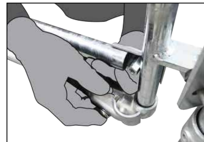
Q. Add clamp onto other end of mid rail, clamping onto the gate upright. Use 6mm hex head socket to tighten supplied M10 bolts into coupling nut.
